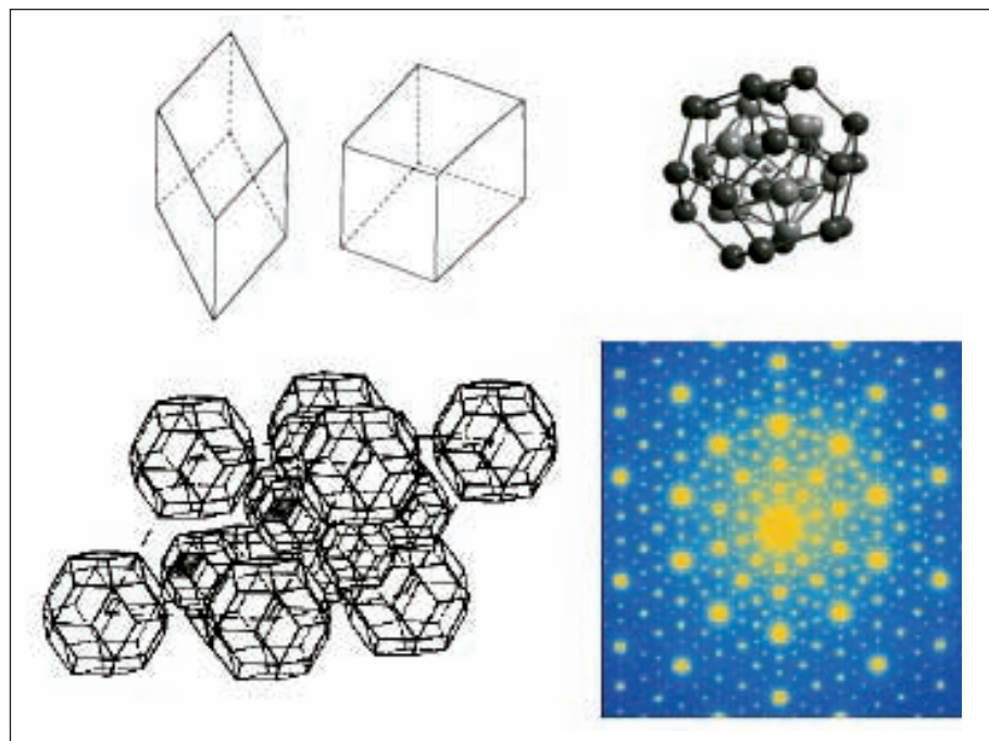
Figure 2. Top left: 3-dimensional Penrose tiles; Top right: An example of the atomic clusters which decorate the vertices of the 3-dimensional Penrose tiling in the model; Bottom left: Schematic of the resulting 3-dimensional cluster structure of the quasicrystal; Bottom right: an electron diffraction pattern from an icosahedral quasicrystal which has 10-fold rotational symmetry. The presence of sharp spots reveals the material has long-range order.
