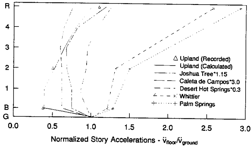
Figure 8: Normalized Accelerations - Calculated and Recorded
