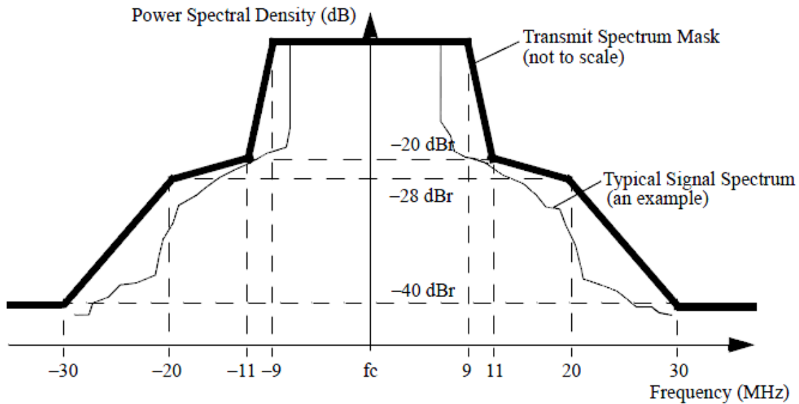
Figure 2: Spectrum mask for WiFi transmissions [5].
